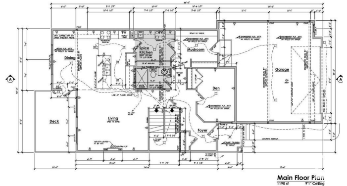
Main Floor Plan 1190 sq ft Ceiling
